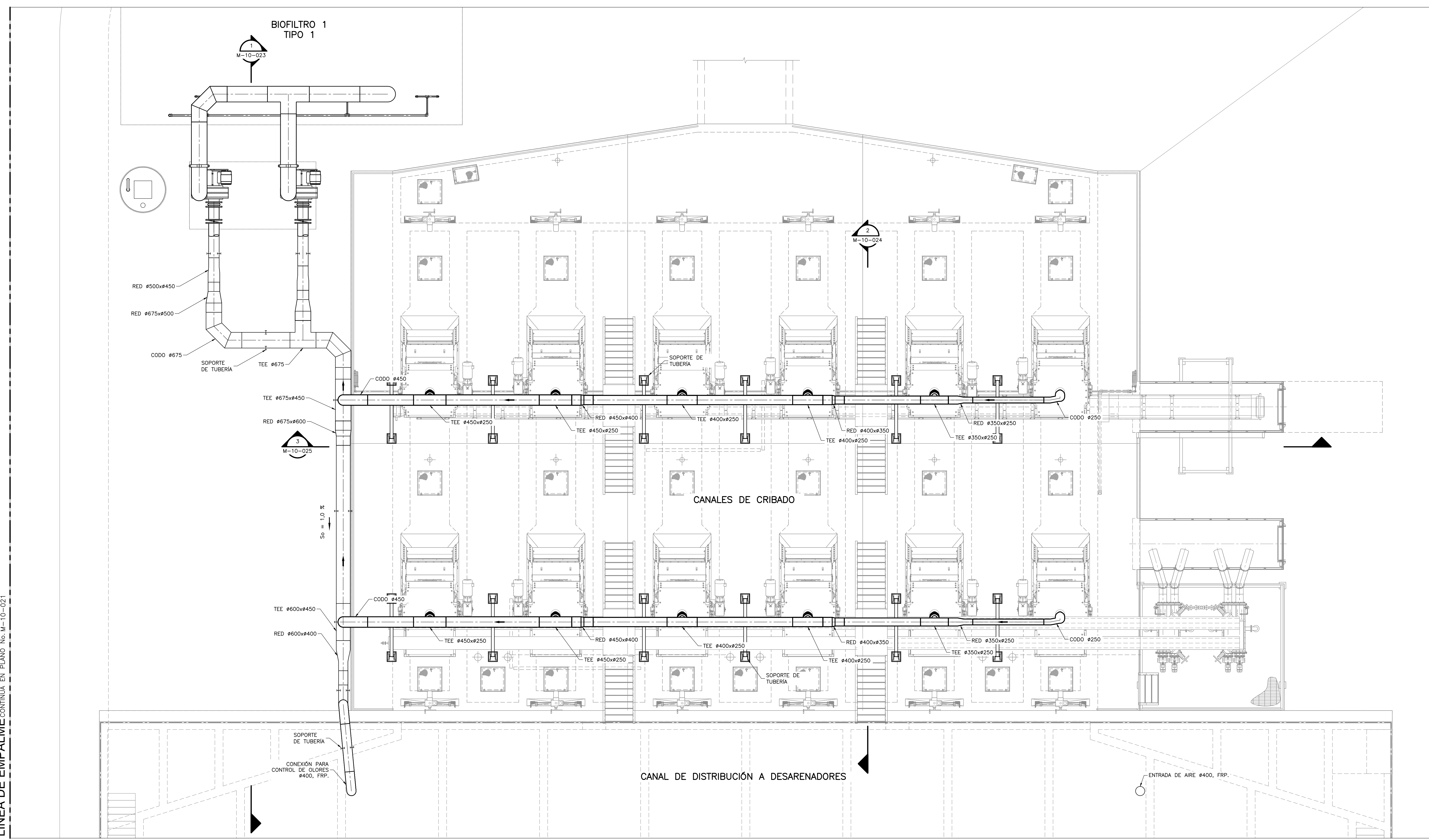
DETALLE B 1=75 M-10-020
