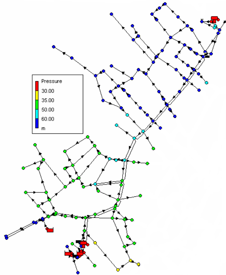
DEMANDA MEDIA
