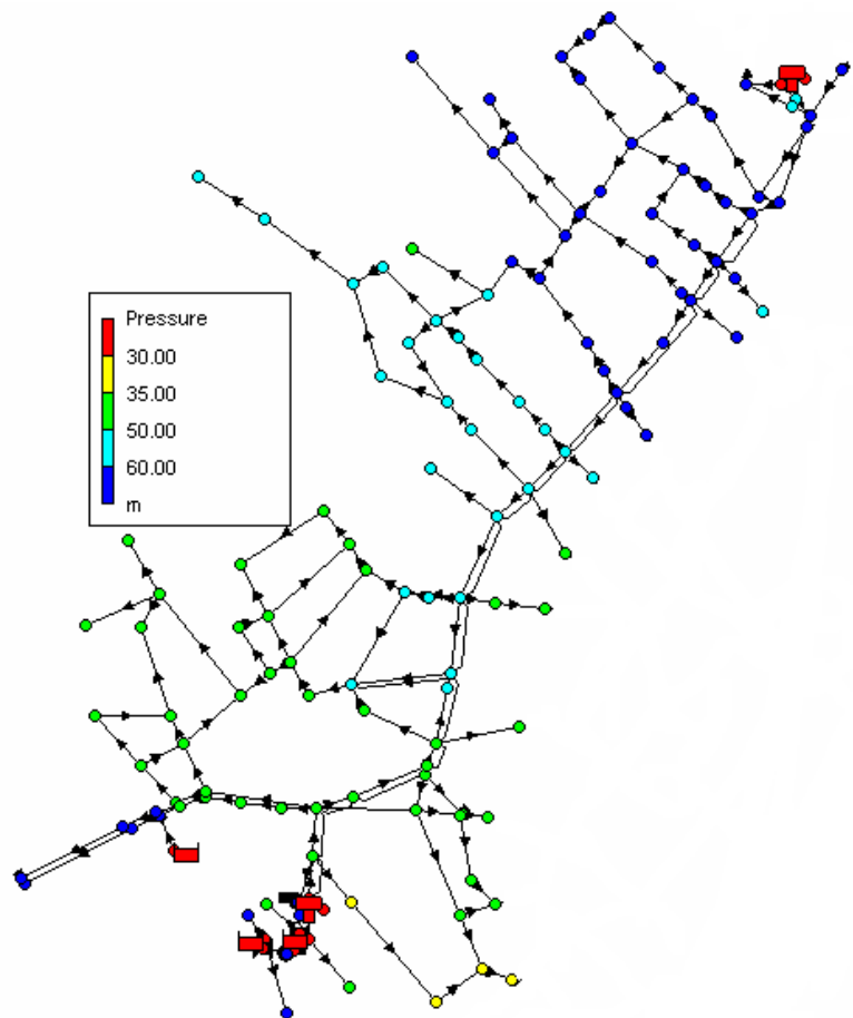
DEMANDA MEDIA
