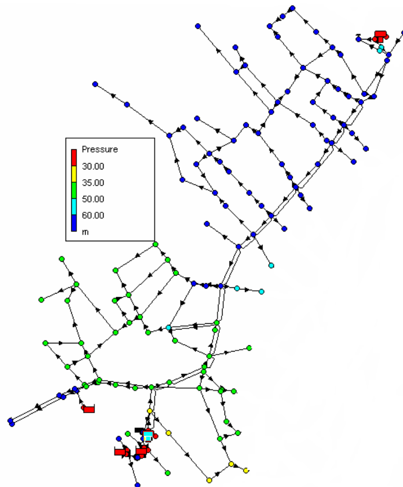
DEMANDA MEDIA
