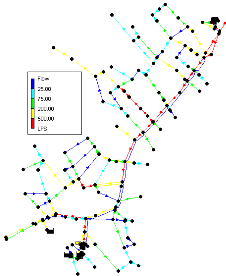
DEMANDA MEDIA
