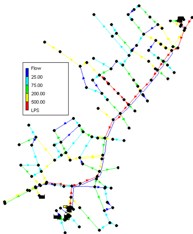
DEMANDA MEDIA
