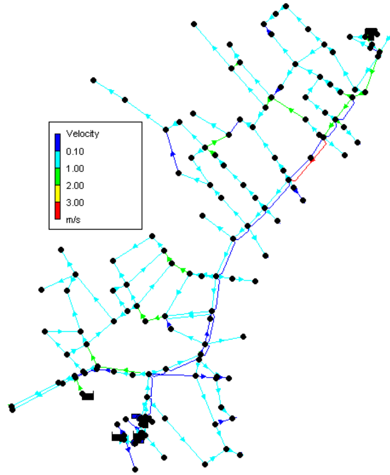
DEMANDA MEDIA
