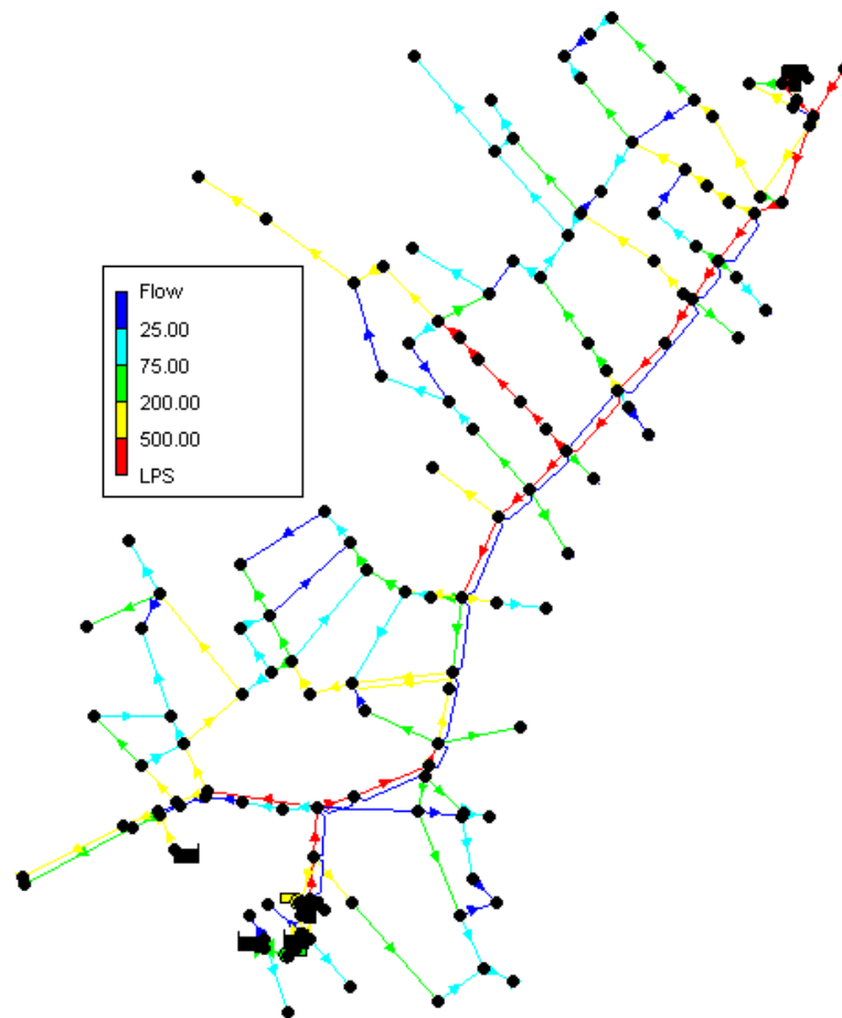
DEMANDA MEDIA
