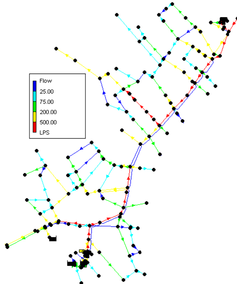
DEMANDA MEDIA
