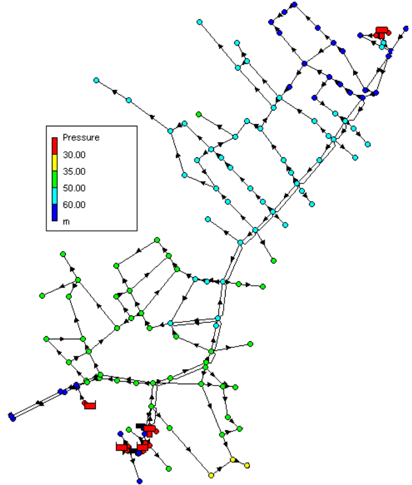
DEMANDA MEDIA
