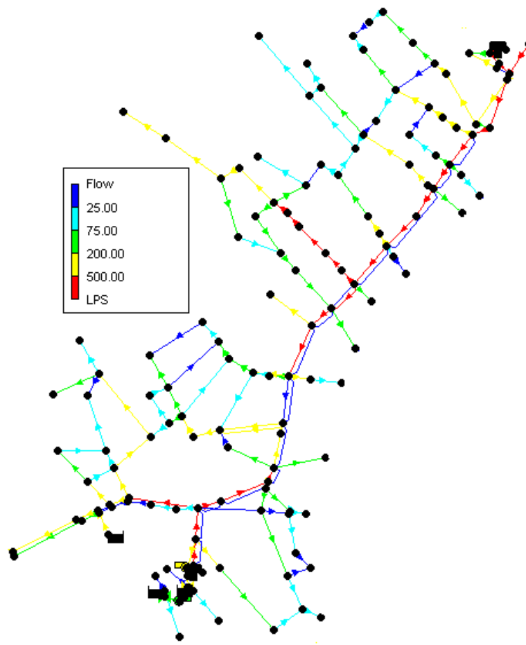
DEMANDA MEDIA
