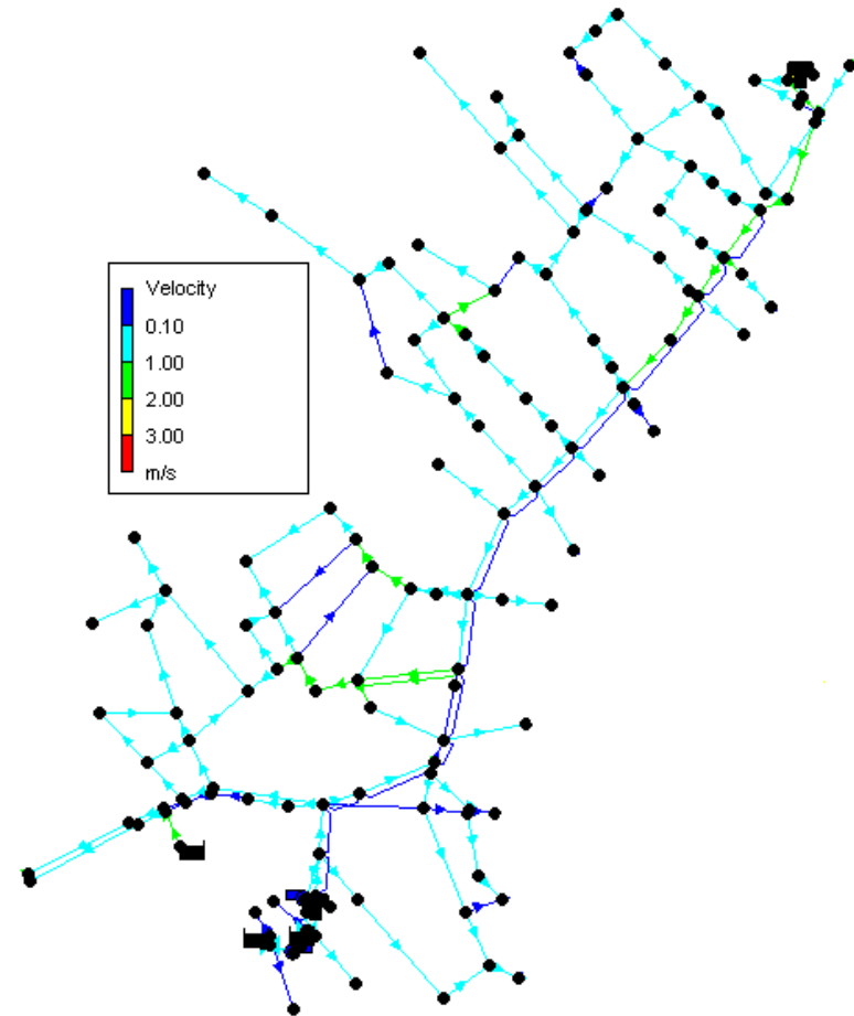
DEMANDA MEDIA
